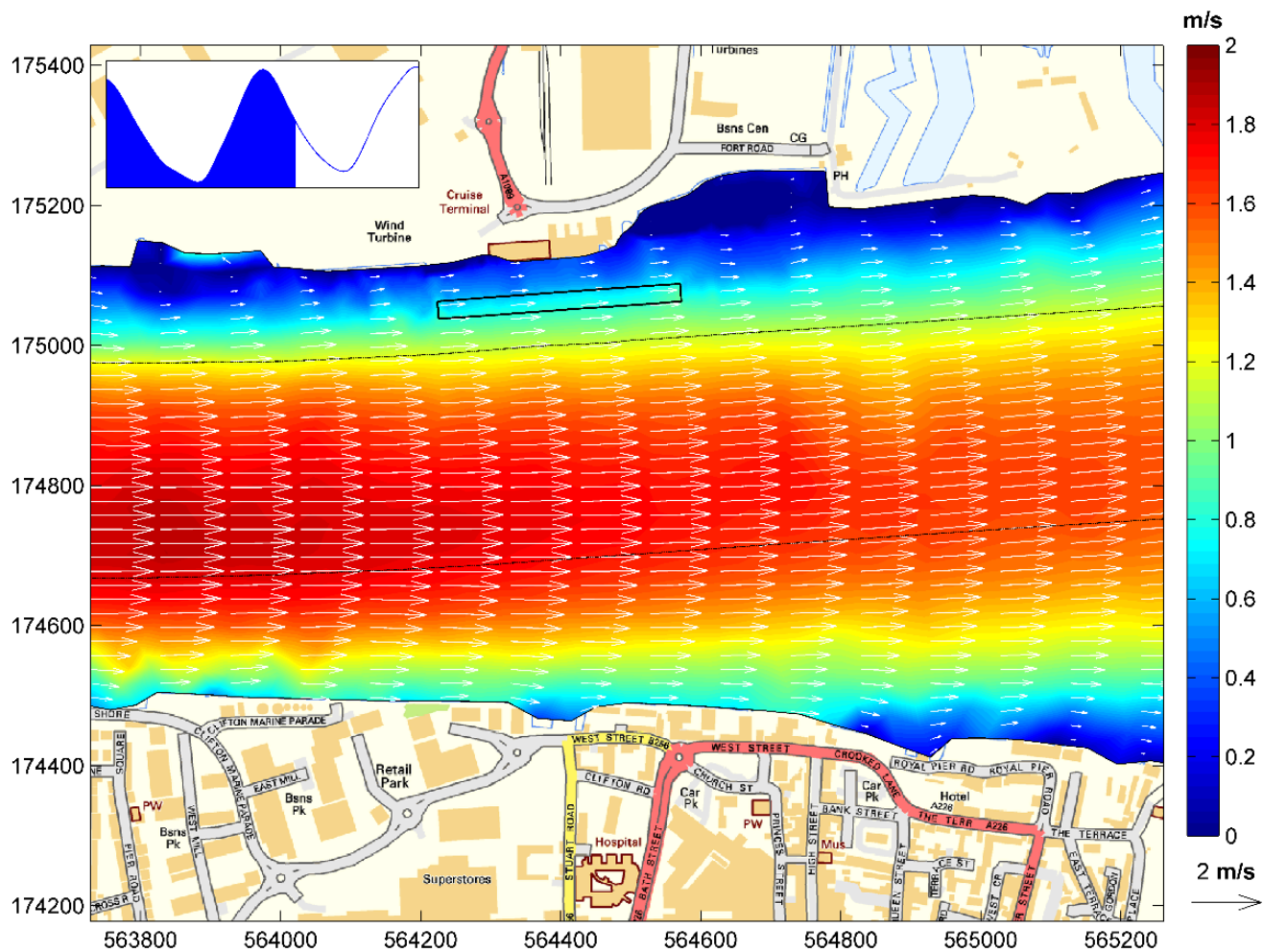
Figure 17.21: Essex Project Site Baseline Hydrodynamic showing current magnitude at time peak ebb tide.
